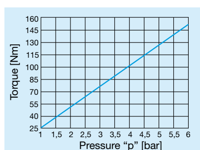
EAS®-Sp 1/45_.125_.
