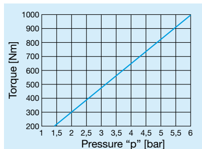
EAS®-Sp 4/45_.125_.
